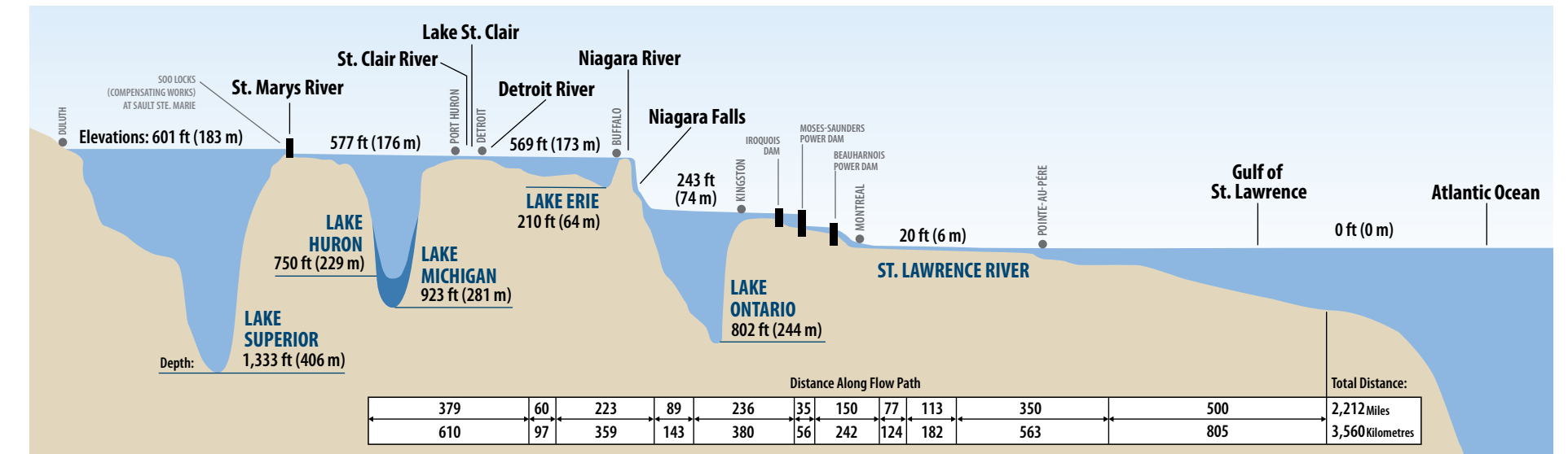
Figure 4: Illustration of Great Lakes surface water level elevations and depths (adapted based on the Michigan Sea Grant illustration )
