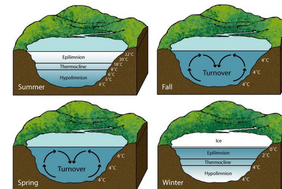
Figure 8: Lake mixing and stratification (credit: Tim Gunther ).
